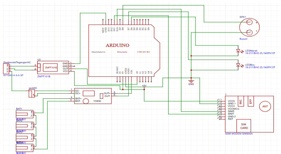
Gambar 3. Schematic diagram alat pendeteksi status listrik
